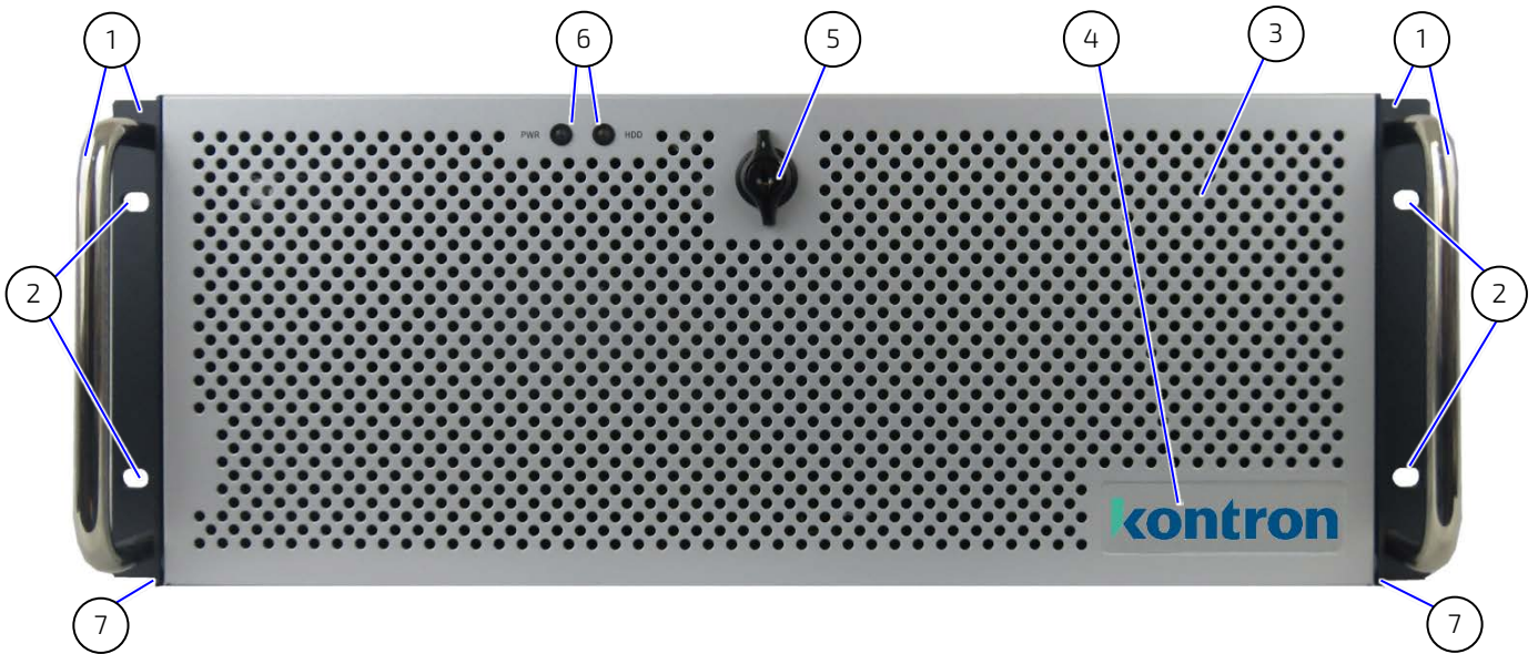
Figure 7: Front Side (front flap closed)
