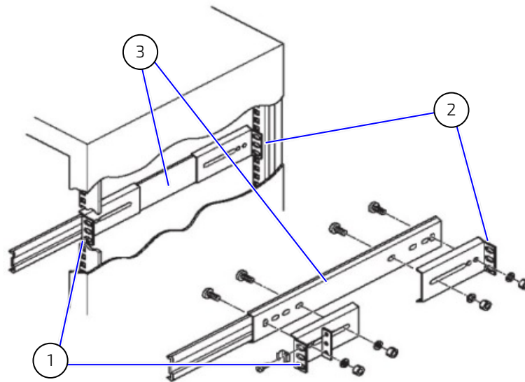
Figure 33: Assembling the Slide Rails in an Industrial Rack Cabinet
