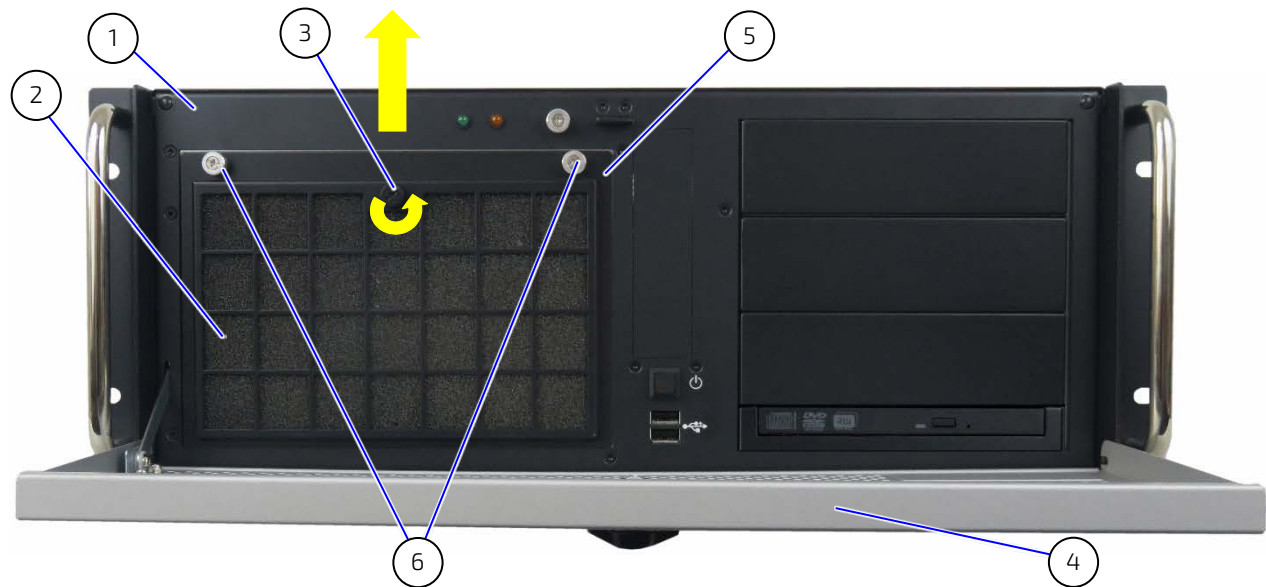
Figure 40: Front Side with Filter Pad Holder
