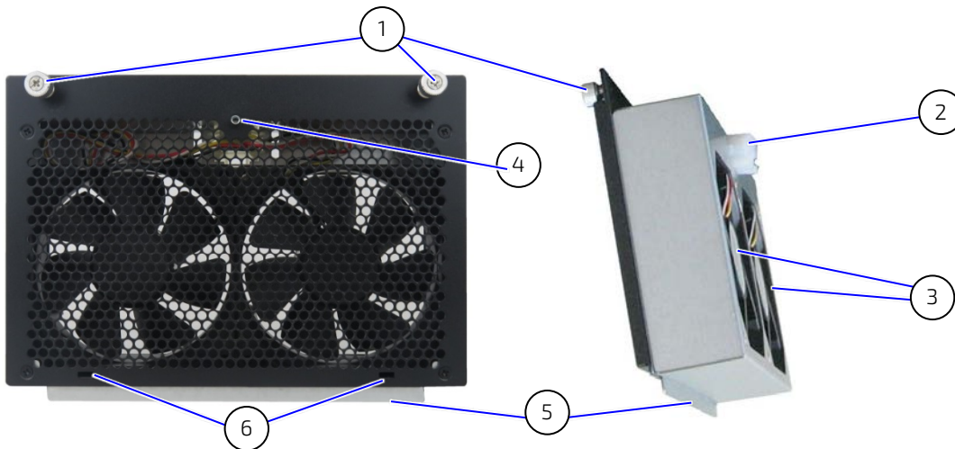
Figure 11: Fan Assembly
