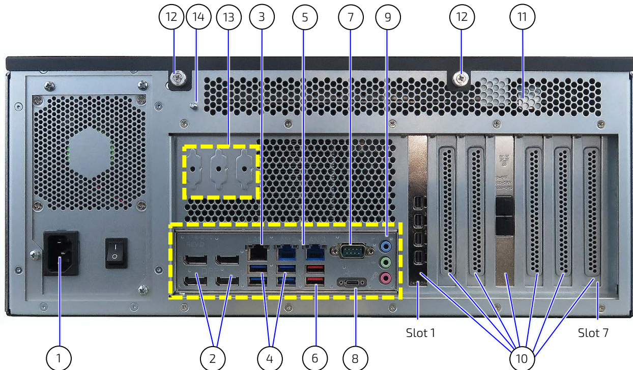
Figure 15: Rear Panel
