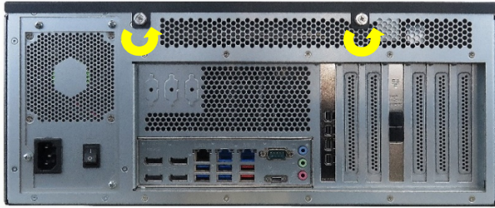
Figure 23: Loosening Knurled Screws (rear panel)
