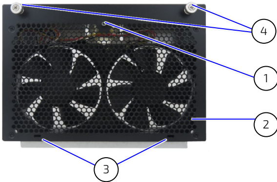
Figure 42: Filter Pad Holder (without filter pad)
