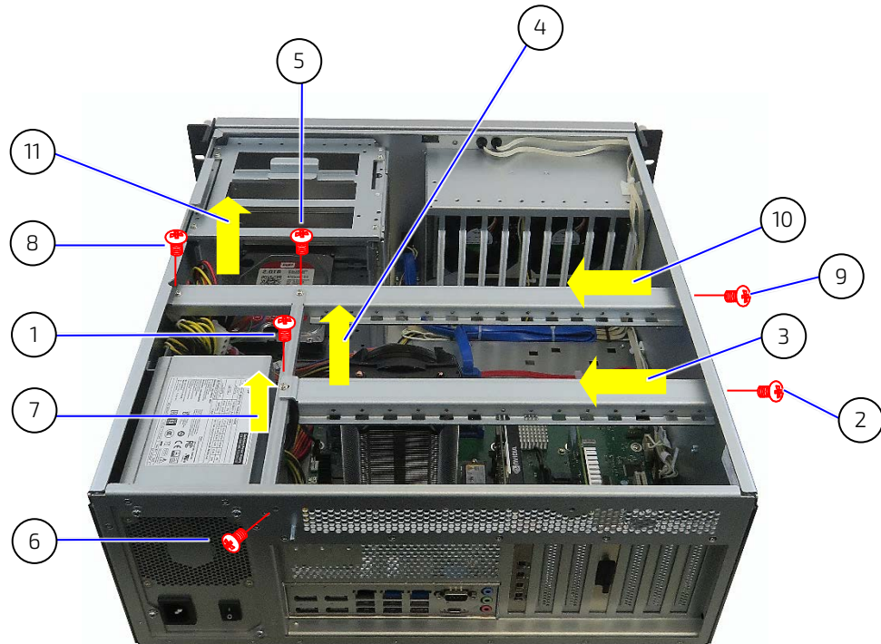
Figure 27: Steps to Remove/Install the Short and Long Brackets
