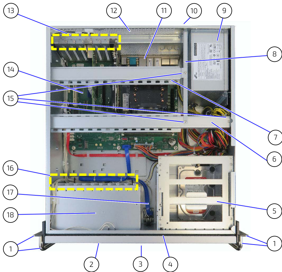
Figure 21: Example of KISS 4U V3 ADL Configuration
