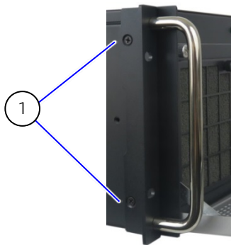
Figure 28: Removing the Handle Brackets
