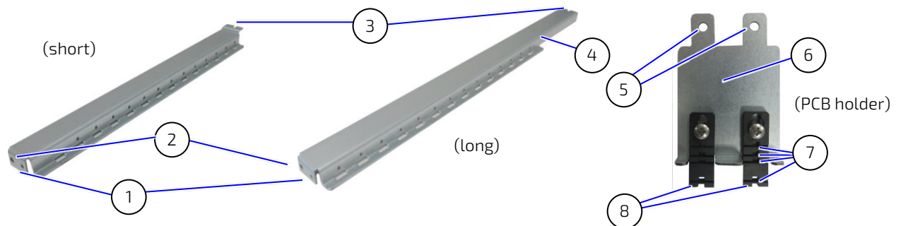
Figure 26: Short and Long Brackets, and PCB Holder
