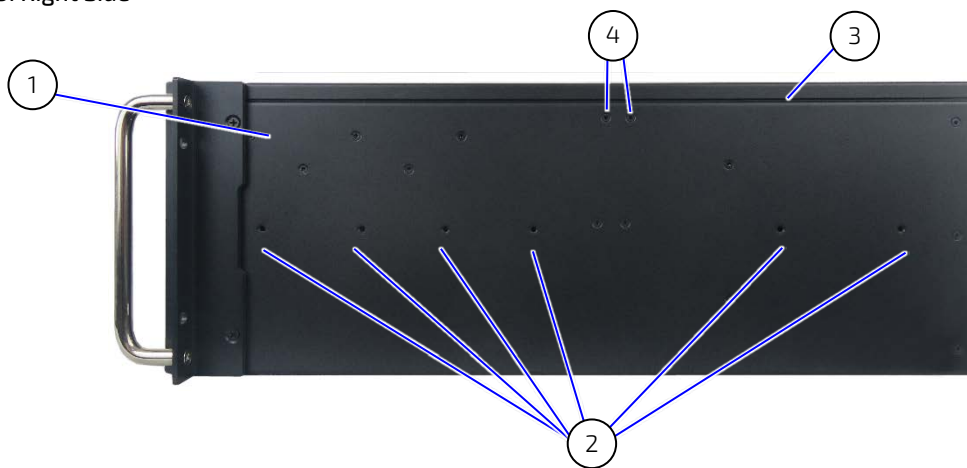
Figure 19: Right Side
