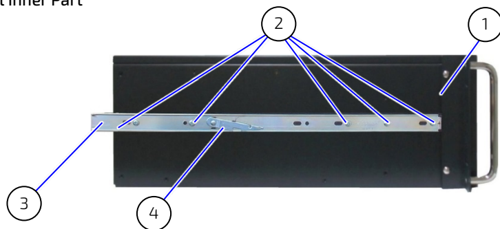
Figure 30: Slide Rail Inner Part
